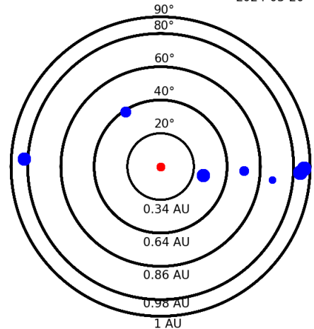
Apparent position of sources in the sky 2024-03-20
