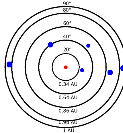
Apparent position of sources in the sky 2024-03-18
