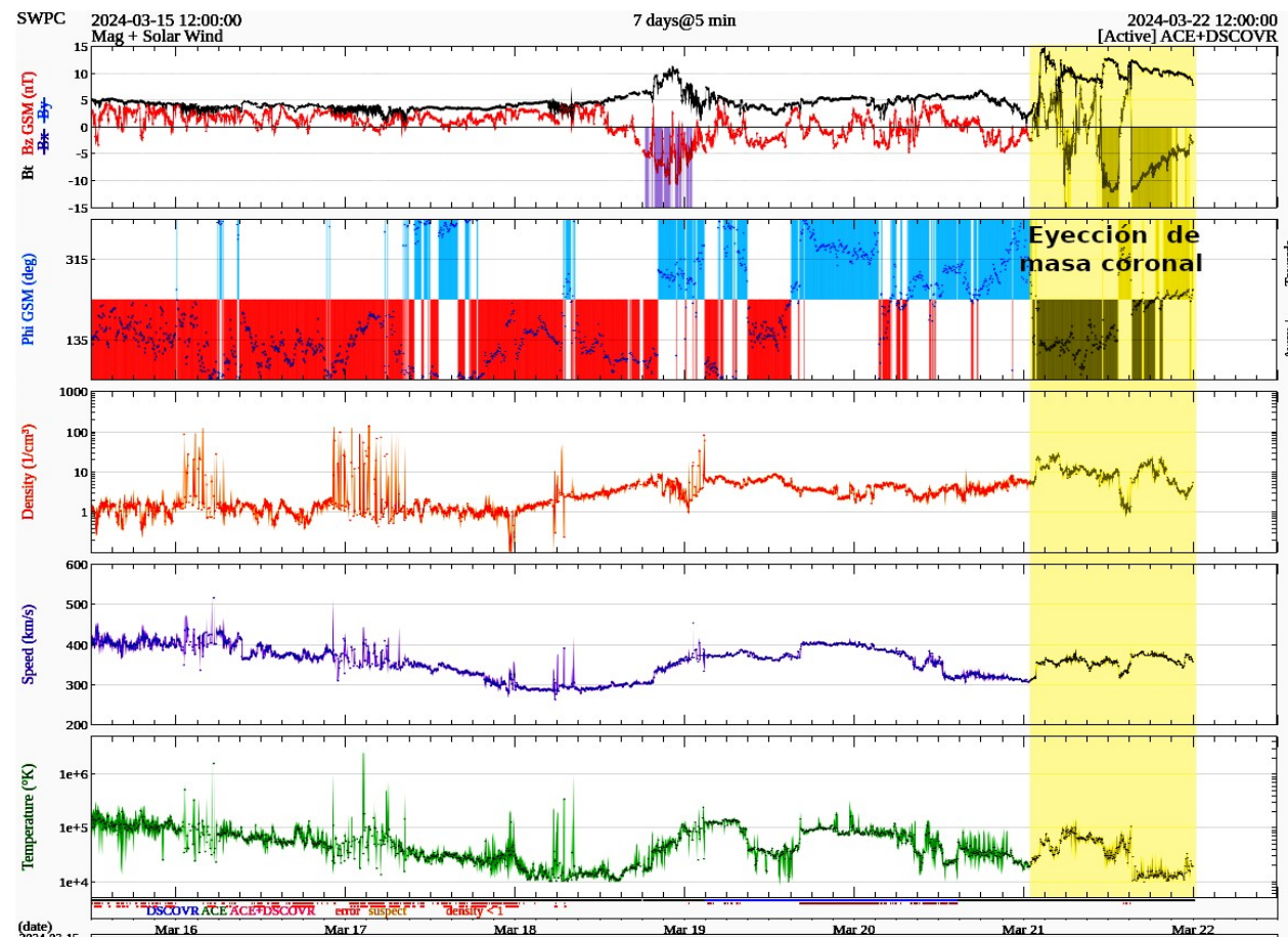
Imagen 2: http://www.swpc.noaa.gov/products/real-time-solar-wind
