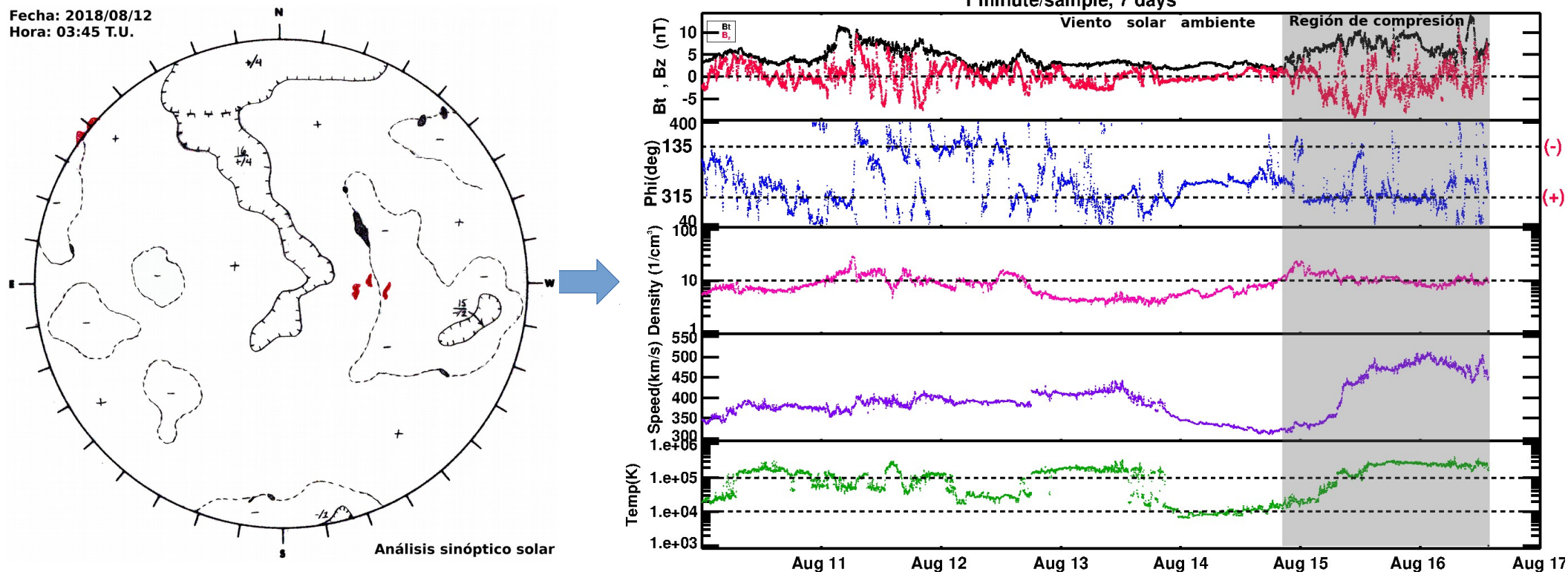
Imagen 1: ftp://ftp.swpc.noaa.gov/pub/synoptic_maps/
