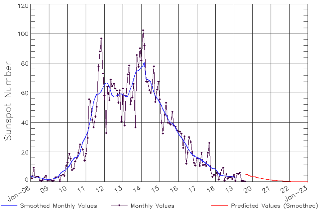
ISES Solar Cycle Sunspot Number Progression Observed data through Aug 2019
