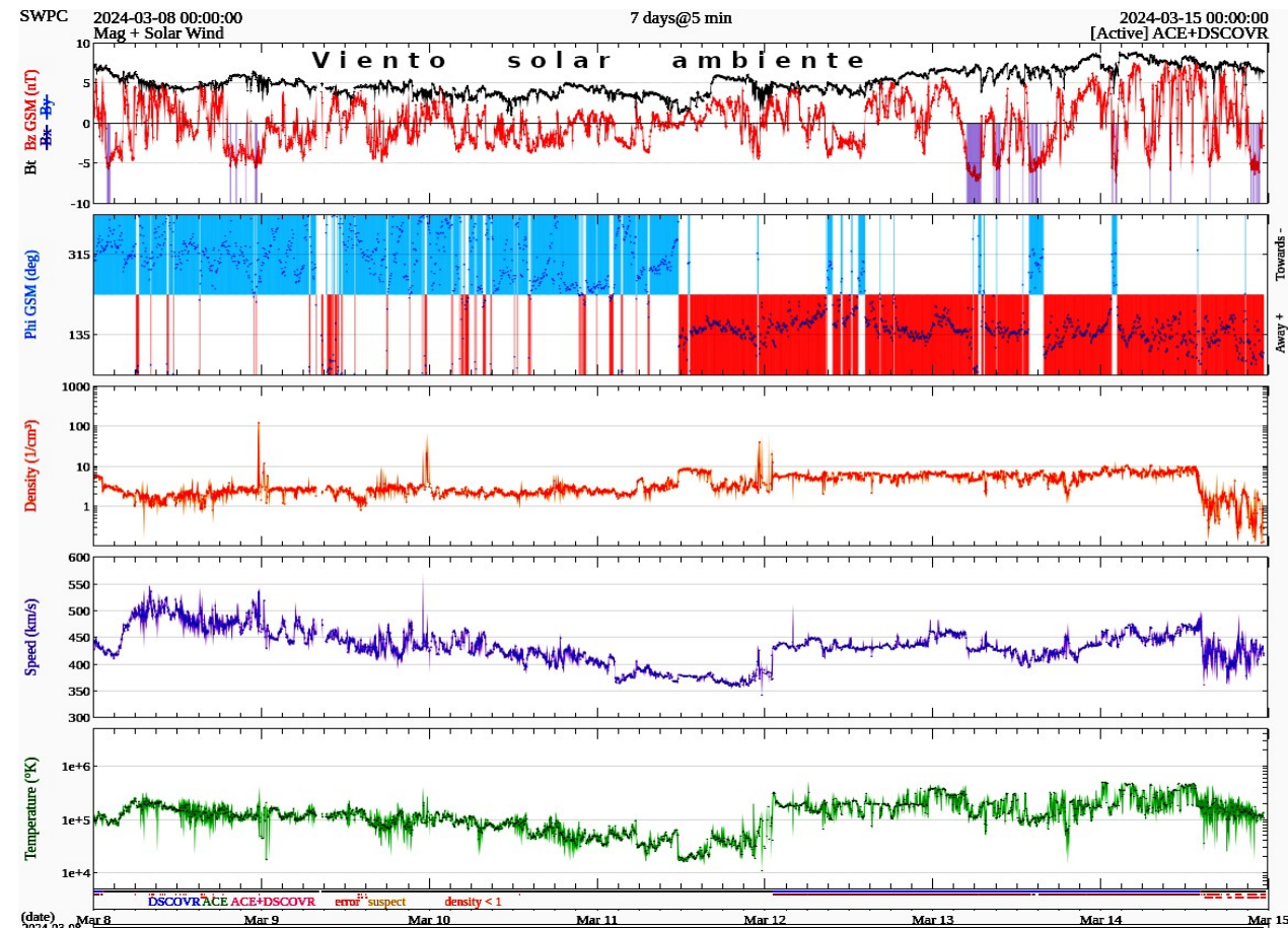
Imagen 2: http://www.swpc.noaa.gov/products/real-time-solar-wind
